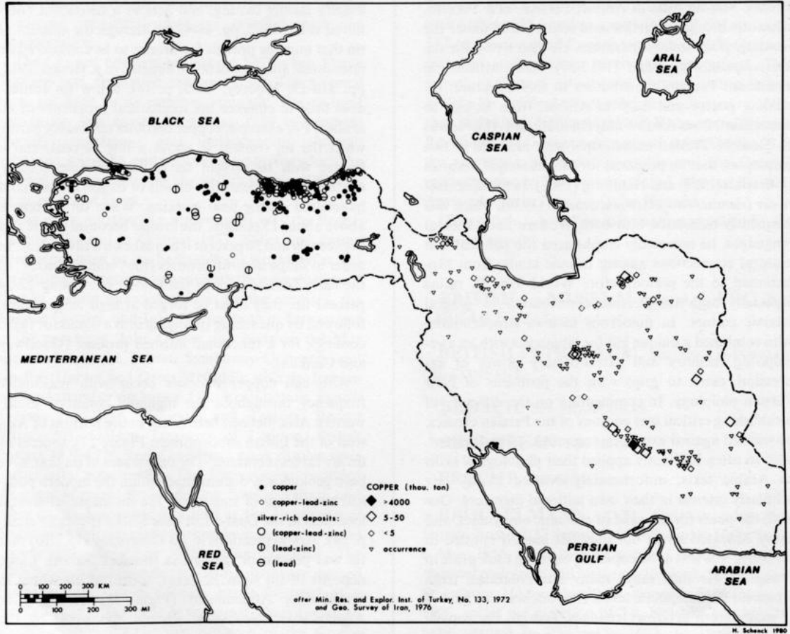
Figure 27. Modern copper ore bodies of Anatolia and the Iranian Plateau
